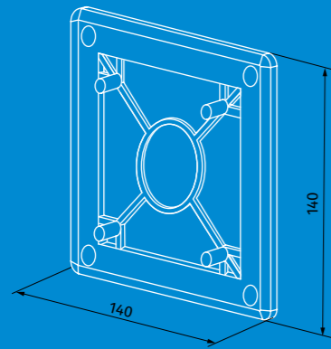
DIMENSIONS [mm]
