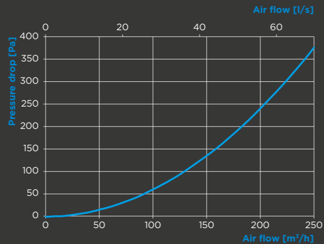
AIR FLOW
