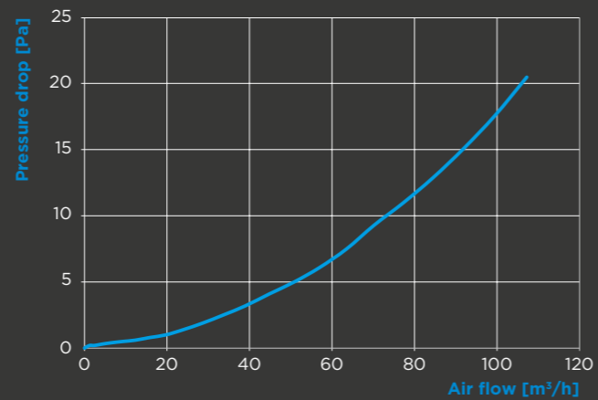
AIR FLOW
