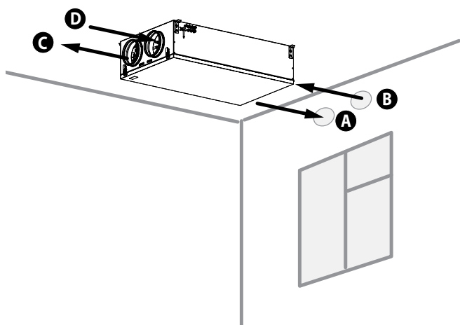
KOMFORT Roto EC D(E) 351(-E) L
