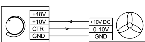
Connection to DC mains with 10 V power voltage
